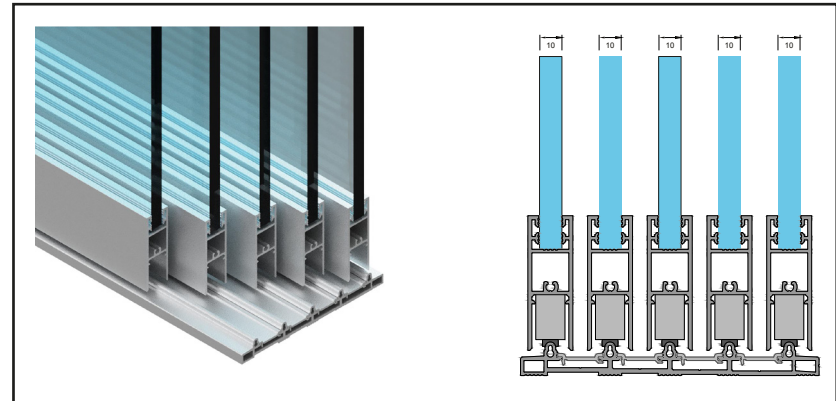
5 Rail System
